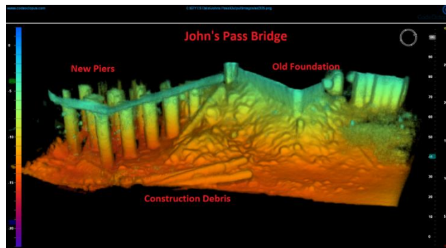
Figure 7: Survey showing broken pilings, shoaling and scour.
